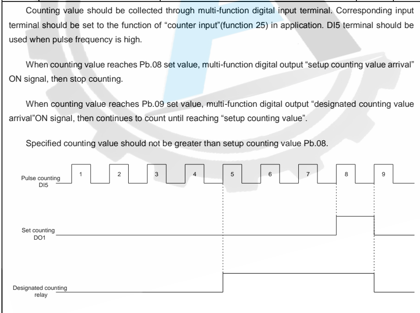
Fig.5-29 Setup counting value&designated counting value schematic diagram
