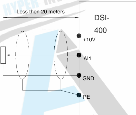
Fig. 2-6.1 Analog input terminal wiring diagram
