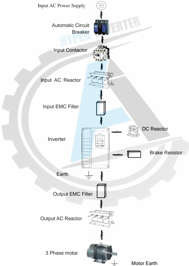
Fig.3-1 Connection diagram of the product and peripheral devices
