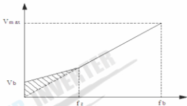
Fig. F5-3 Torque Boost
