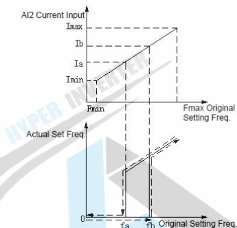
Fig. F6-1 zero-frequency function schematic diagram
