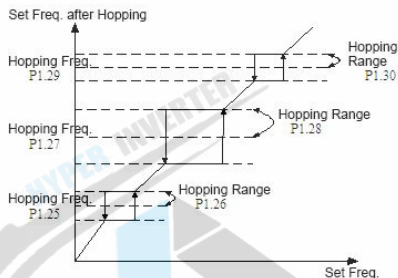
Fig. F1-6 Hopping Frequency
