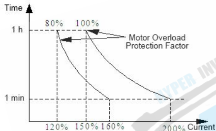
Fig. FA-2 Motor Overload Protection Factor Setting
