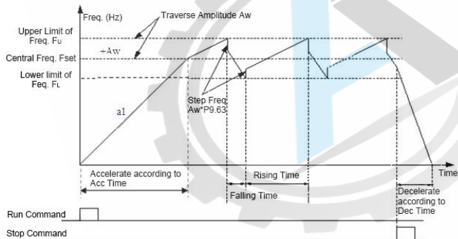
Fig.F9-6 Traverse Operation
