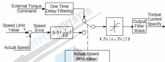
Figure F4-2 Torque Control Simplified diagram
