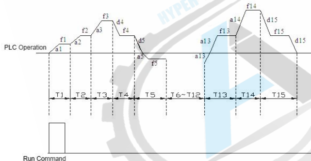
Fig. F9-1 Stop after a Single PLC Cycle
