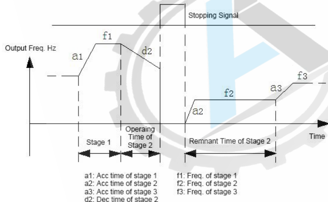
Fig. F9-4 PLC Start Mode 1
