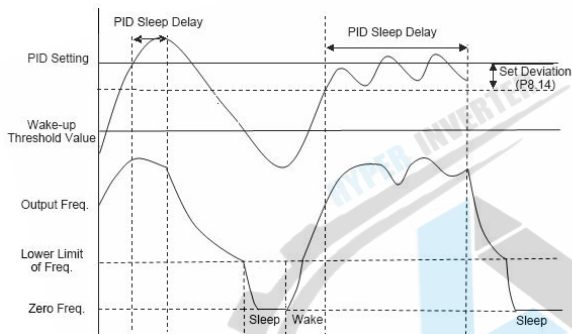
Fig. F8-6 the Second Sleep Mode
