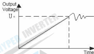
Fig. F5-5 Voltage Control Mode 1
