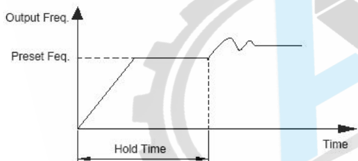
Fig. F8-4 Closed Loop Preset Frequency
