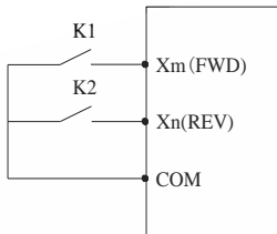
Fig. F7-3 2-wire Control Mode 2
