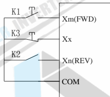
Fig. F7-5 3-wire control mode 2
