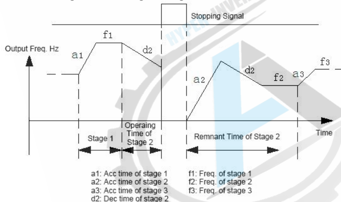
Fig.F9-5 PLC Start Mode 2
