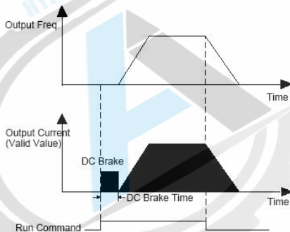
Figure F1-2 start DC brake
