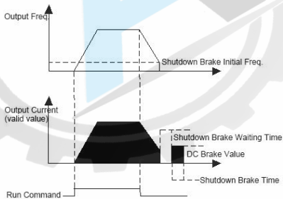
Fig. F1-4 Stop DC Braking
