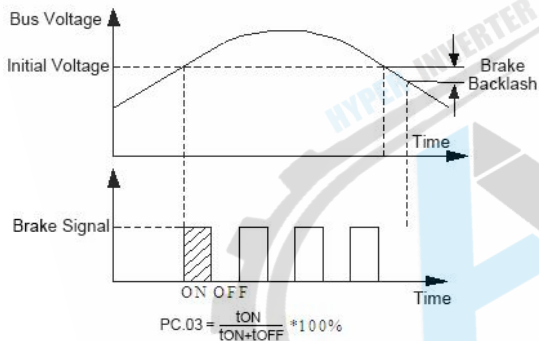
Fig. FC-1 Dynamic Braking
