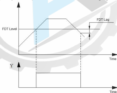
Fig.F7-8 Frequency Level Detecting
