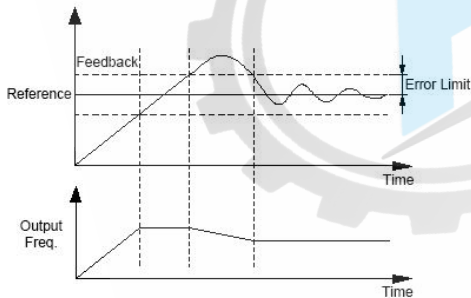
Fig. F8-3 Error Limit Schematic Diagram
