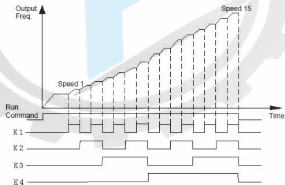
Figure F7-1 Multi-speed Running
