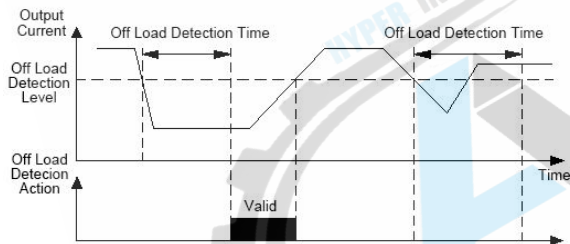
Fig. FA-3 Off Load Detection
