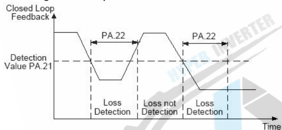
Fig. FA-4 Closed Loop Feedback Loss Detection
