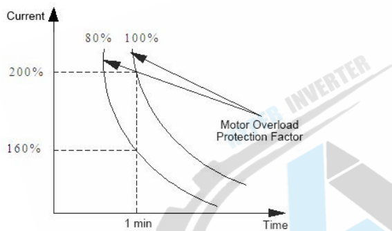
Fig.FA-1 Motor Overload Protection Factor
