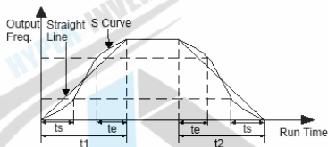
Fig. F1-3 Straight Line and S Curve of Acc./Dec.
