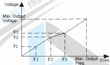
Fig. F5-2 User Setting V/F Curve
