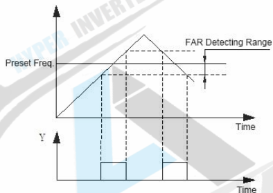
Fig. F7-7 Frequency Arrival
