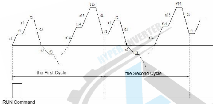
Fig.F9-3 PLC Continuous Cycle
