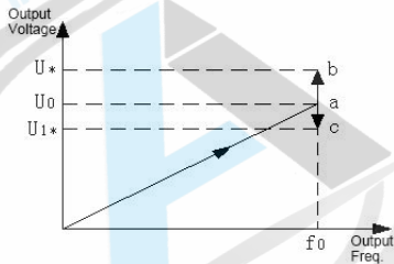
Fig. F5-4 Voltage Control Mode 0
