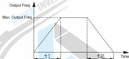
Figure F0-2 Accelerating and Decelerating time
