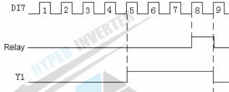
Fig. F7-9 Counter Reset and Detection Setting
