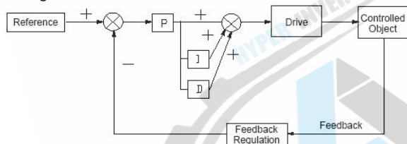
Fig. F8-2 PID Regulation
