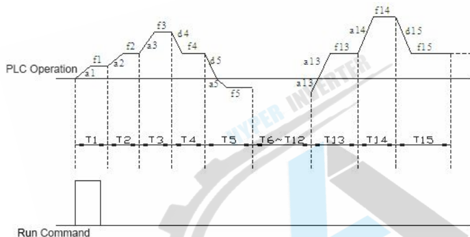
Fig.F9-2 Maintain Last Stage after Single Cycle
