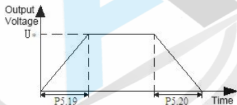
Fig. F5-7 Voltage Control Mode 2
