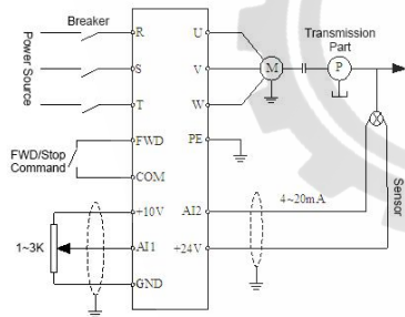
Fig. F8-1 Analog Feedback Control System
