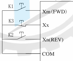
Fig. F7-4 3-wire Control Mode 1
